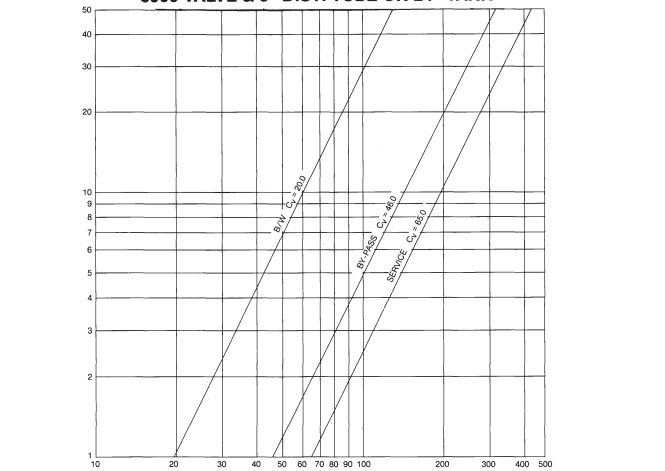
3900 VALVE & 3" DIST. TUBE ON 24" TANK
